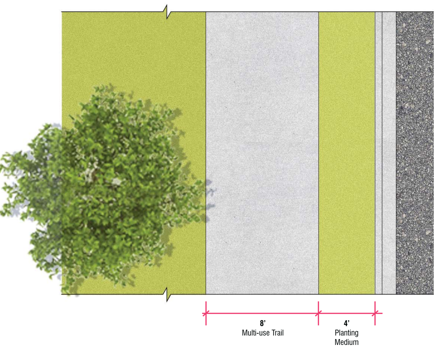
Typical Riverfront Trail Plan
