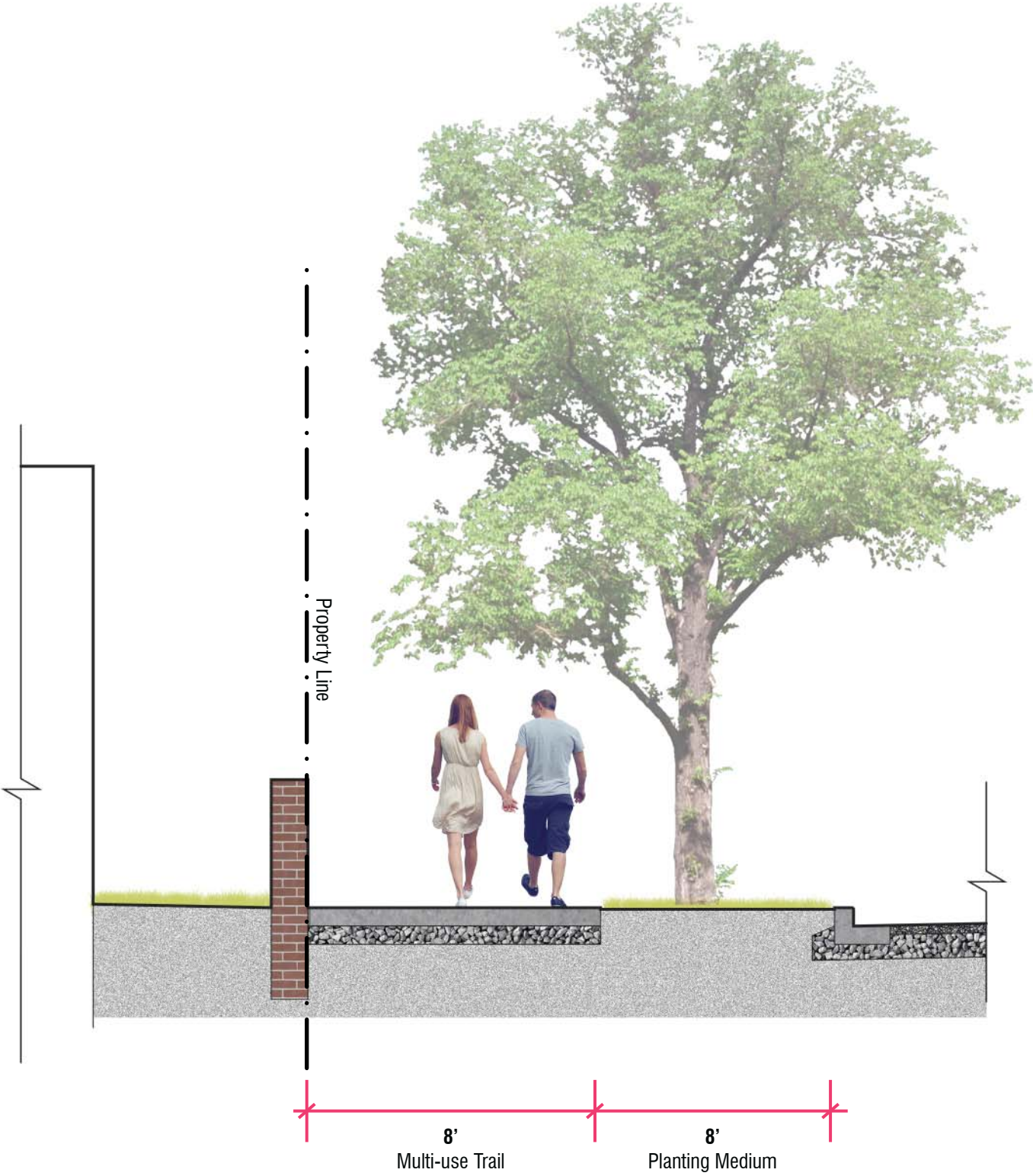
Typical Residential Trail Section
