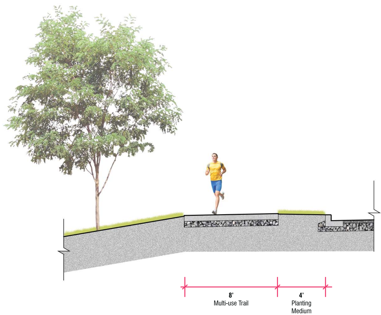
Typical Riverfront Trail Section
